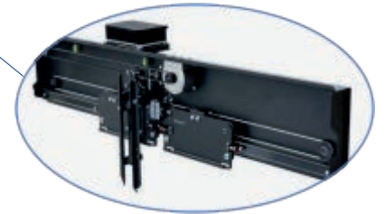
Advanced car door mechanical lock and door safety edge 現代化機廂門鎖及門刀
